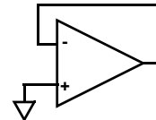
FIGURE 42. PREVENTING OSCILLATIONS IN UNUSED CHANNELS
